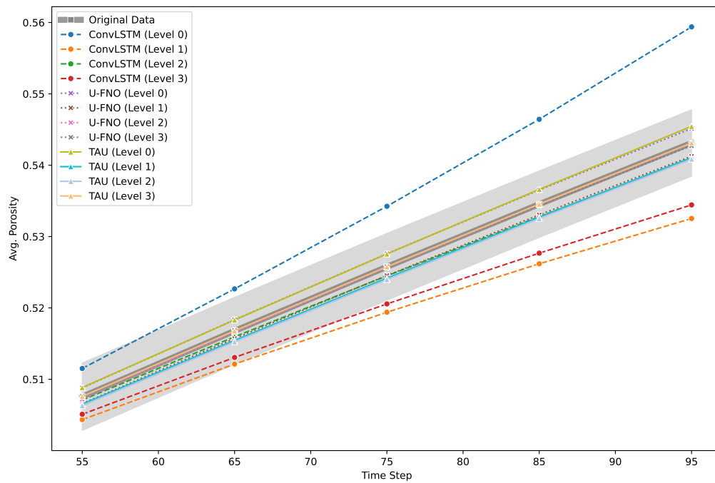
(a) Absolute Porosity Evolution (Validation Set)
