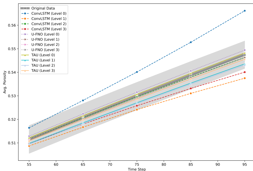
(a) Absolute Porosity Evolution (Training Set)
