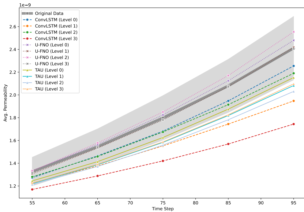
(a) Average Permeability Evolution (Validation Set)
