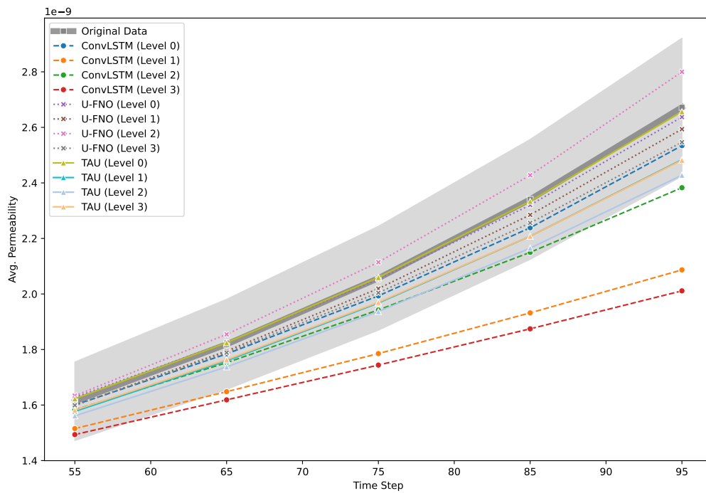
(a) Absolute Permeability Evolution (Training Set)
