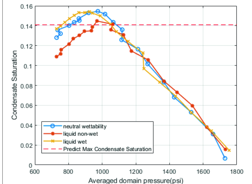
Figure 11: Condensate saturation versus averaged domain pressure at different wettability conditions (neutral, liquid non-wet, and liquid wet) in the VT porous medium. According to thermodynamic predictions, the maximum condensate saturation at equilibrium is 0.140.
