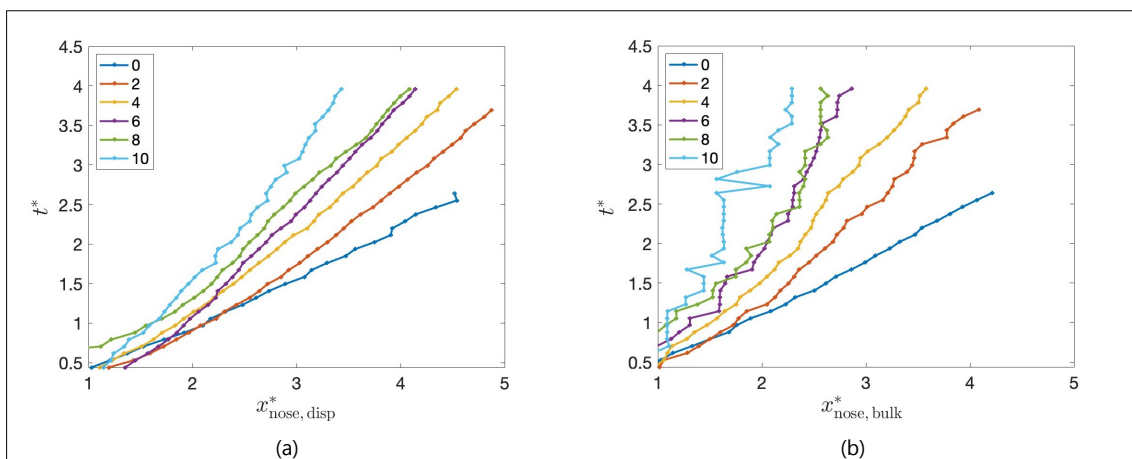
Figure 10: Time evolution of the gravity current front as characterized by the (a) dispersed phase, x_{nose, disp}^* and (b) bulk phase, x_{nose, bulk}^* . Here we consider the same set of experiments from Figures 5, 7, 8 and 9 . The greater scatter observed in (b) for large \mathcal{N} is a consequence of the gravity current becoming very thin and therefore harder to visualize in experimental images -- see e.g. Figure 7 .
