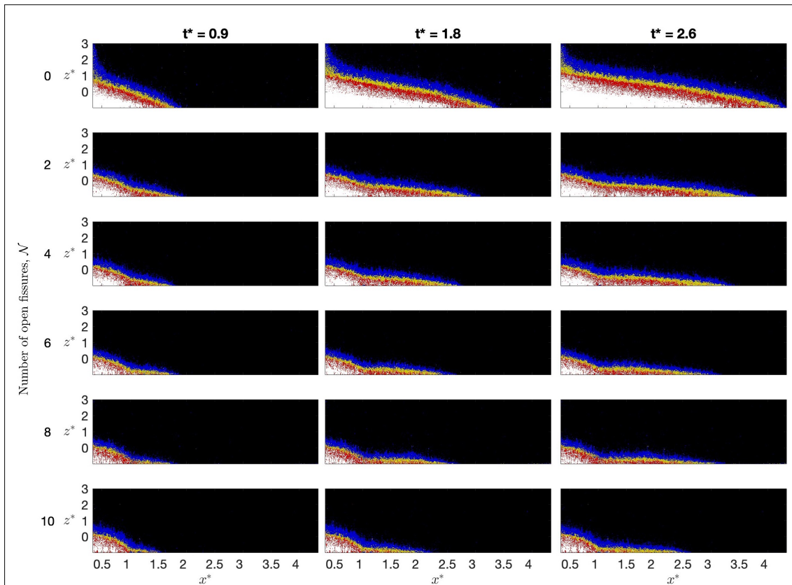
Figure 5: Collage image showing the time evolution of six different experiments (i.e. E1, E5, E9, E13, E17 and E21), each corresponding to a different number of open fissure holes. The spatial coordinates x^* and z^* are defined by Equation 5 where x^* = 1 shows the fissure location. Colored shading is applied over the following range of normalized saline concentrations: black -- 0 to 0.10; blue -- 0.10 to 0.25; yellow -- 0.25 to 0.50; red -- 0.50 to 0.75; and white -- 0.75 to 1.
