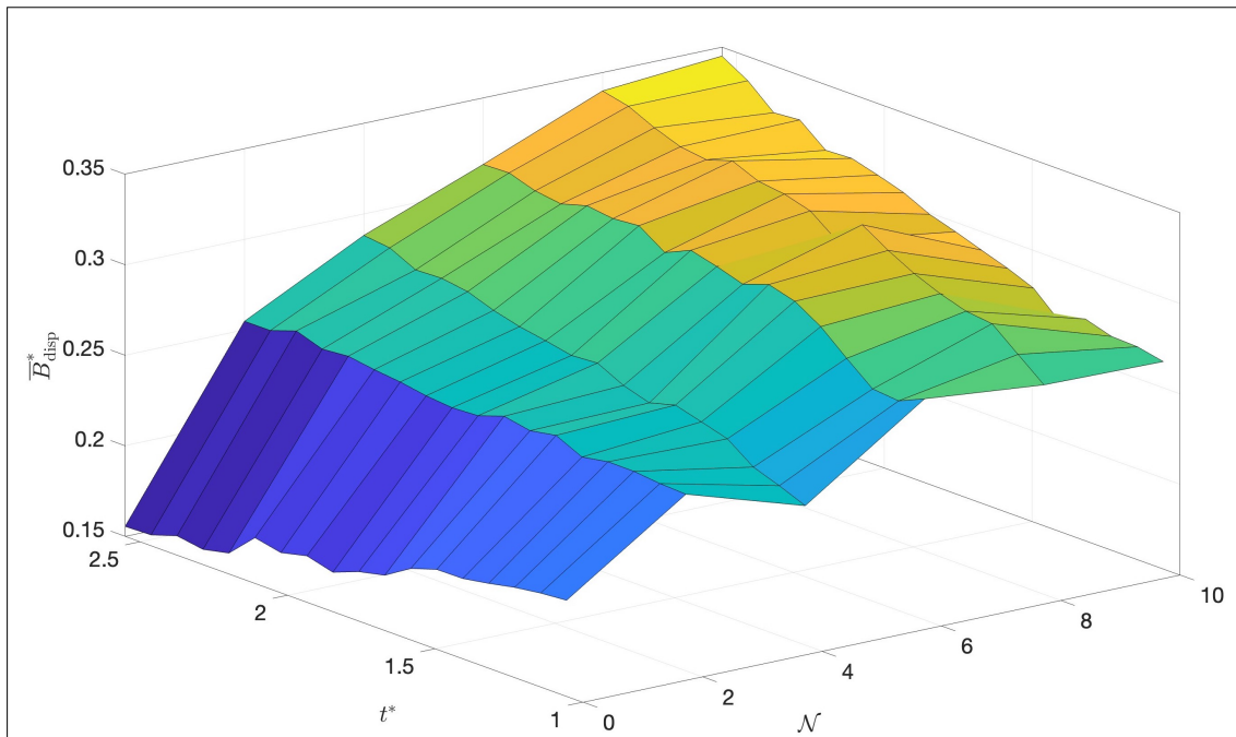
Figure 9: Dispersed buoyancy fraction versus time and \mathcal{N} . Here we consider the same set of experiments from Figures 5, 7, and 8 .
